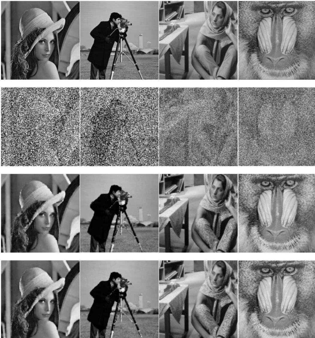
Fig. 2 From top to bottom: original images, noisy images with 0.7 the salt-and-pepper noise, the restorations obtained by minimizing \mathcal{F}_\alpha with TPRP method and Algorithm 1, respectively.
