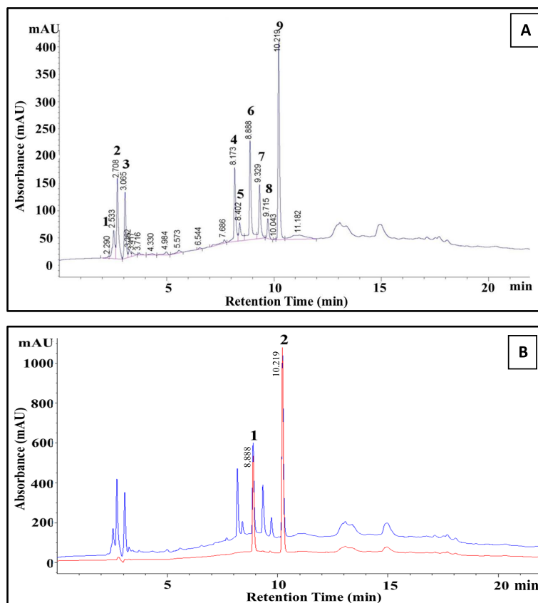
Fig. 1 Ultra-high performance liquid chromatograms of A. esculentus extract (A). The chromatograms of mixed standards, rutin (1) and quercitrin (2) overlapped on the A. esculentus extracts chromatograms (B).
