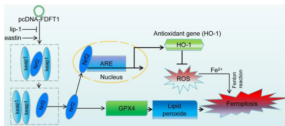
Fig. 6 Schematic summarizing mechanism of FDFT1 in regulating ferroptosis in this study.
